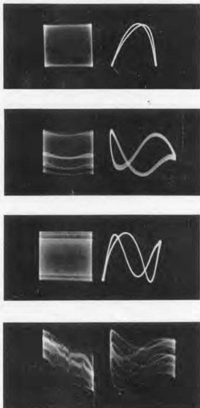
Figure 3. Typical distortion and hum patterns. In each case the pattern on the left is produced with power-line-frequency synchronization, the pattern on the right with signal-frequency synchronization.
